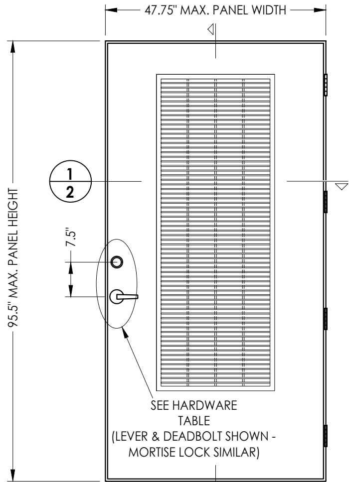
40 VENTED DOOR PANEL
